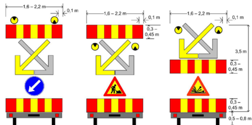
Figure 4.5 Examples of warning panels, large size.
