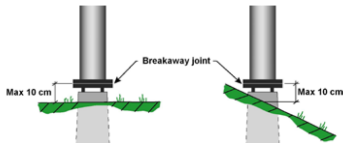
Figure 5.9 Installation of breakaway joint
