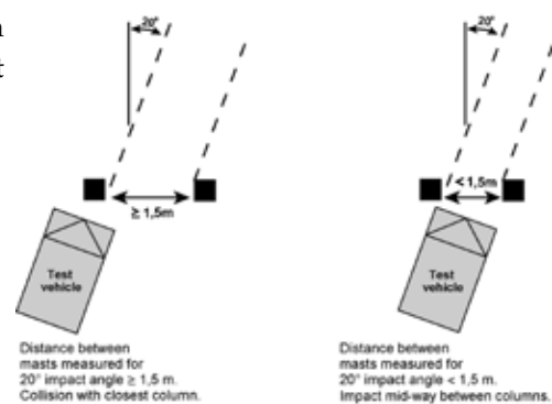
Figure 5.10 Requirements regarding inter-column distance.
