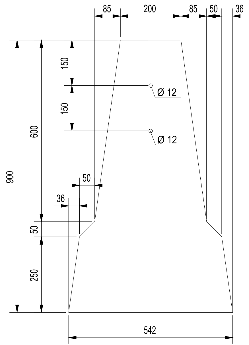
VS H2 D90 SCALE 1:10
