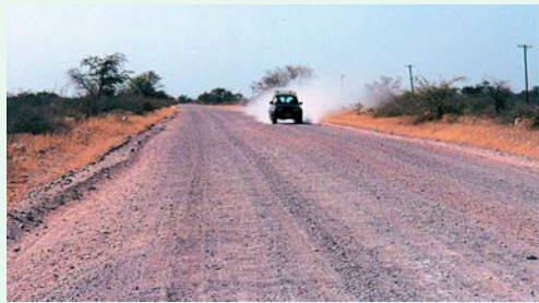
Unsealed roads very often corrugate, resulting in a rough surface and associated high maintenance and operational costs.
