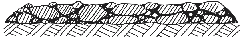
Single Otta Seal (0-16 mm). Thickness: minimum 16 mm
