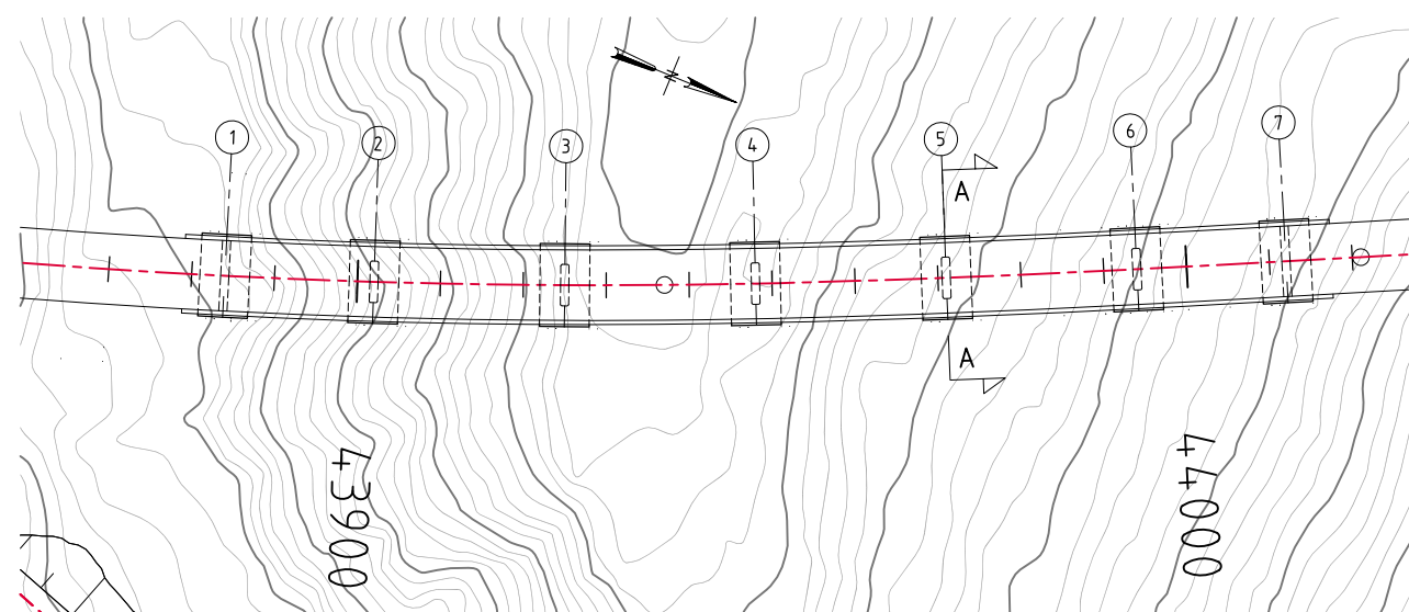
PLAN 1:500
